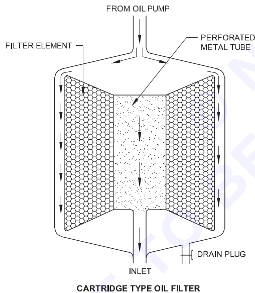
CARTRIDGE TYPE OIL FILTER
