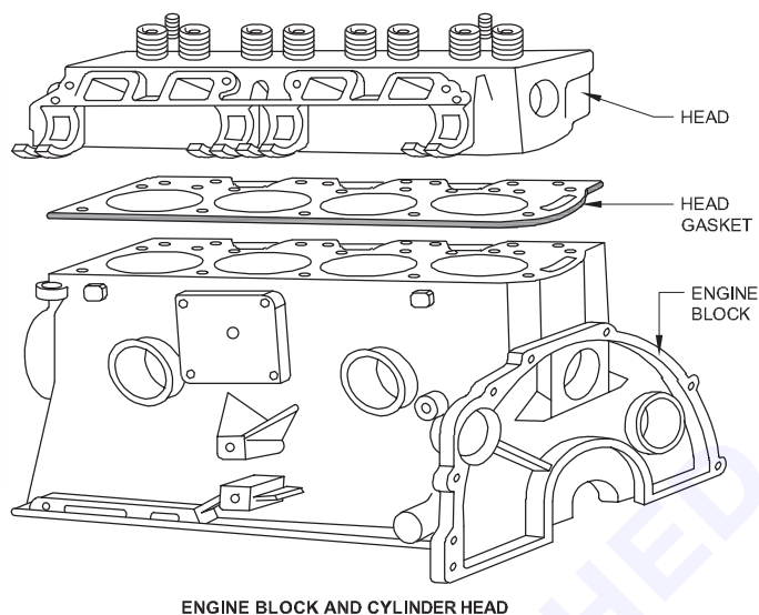
ENGINE BLOCK AND CYLINDER HEAD
