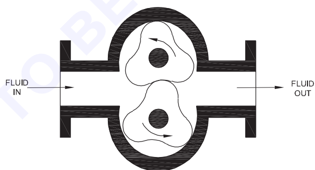
FLUID TRANSFER THROUGH ENGAGED ROTATION LOBES
