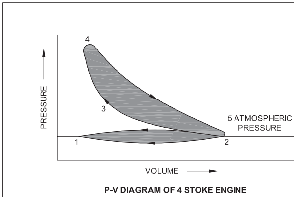
P - V Diagram of 4 stroke engine
