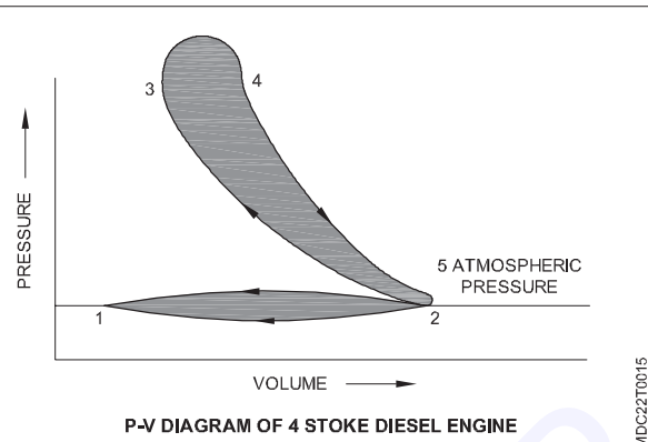
P-V Diagram of 4 stroke diesel engine
