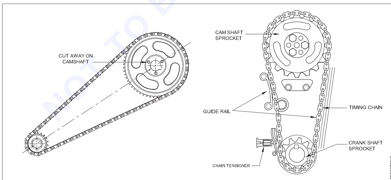
Valve timing chain type
