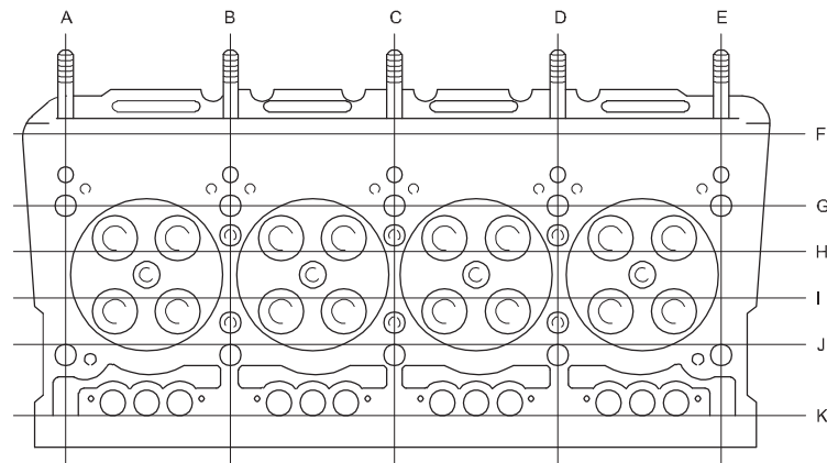
POSITION FOR CHECKING CYLINDER HEAD FOR FLATNESS
