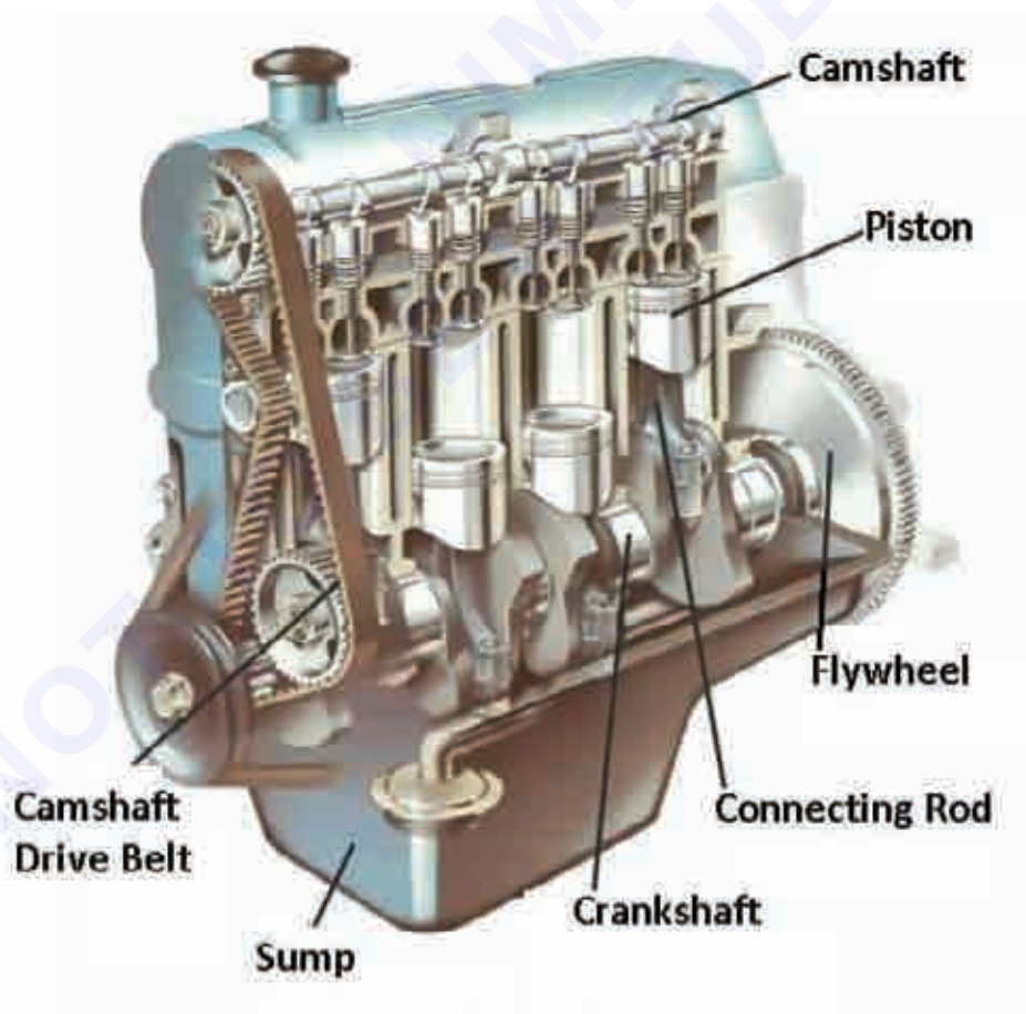
Four-stroke compression-ignition engines-ii (Perkins)
