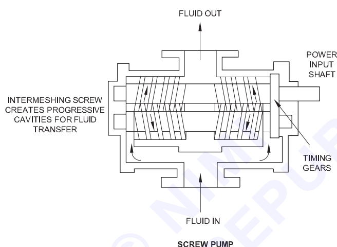
SCREW PUMP
