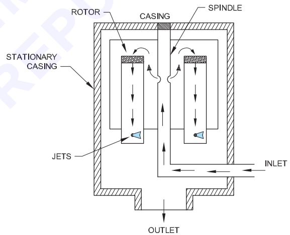
CENTRIFUGAL TYPE OIL FILTER
