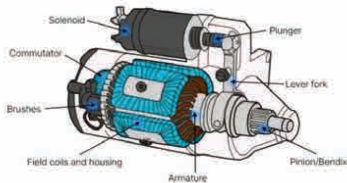
Starter Motor Parts
