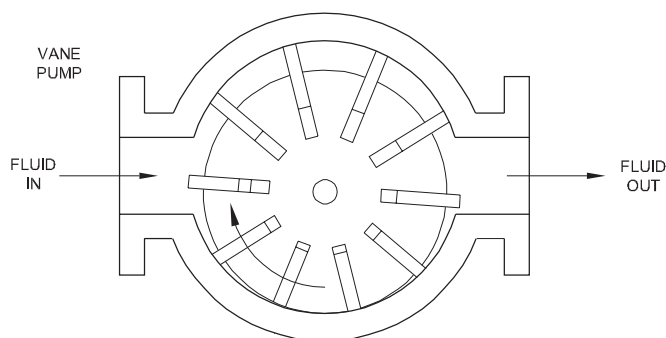
FLUID GET TRAP &amp; TRANSFER BY SLIDING / ROTATING VANES
