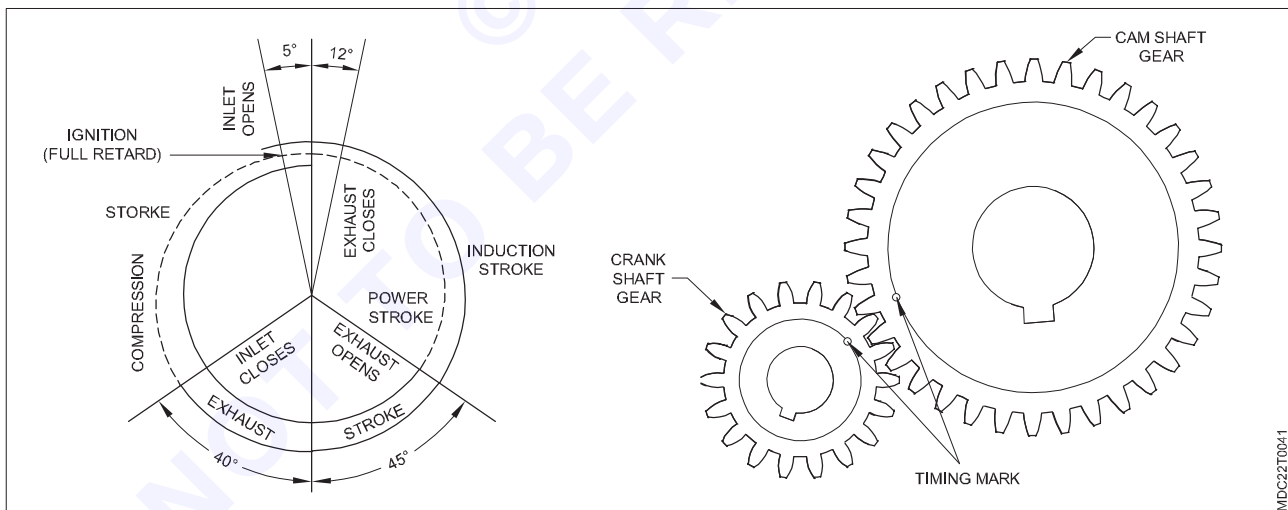
Valve timing on crankshaft rotation
