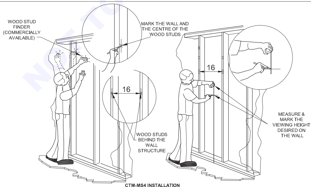
CTM-MS4 INSTALLATION
