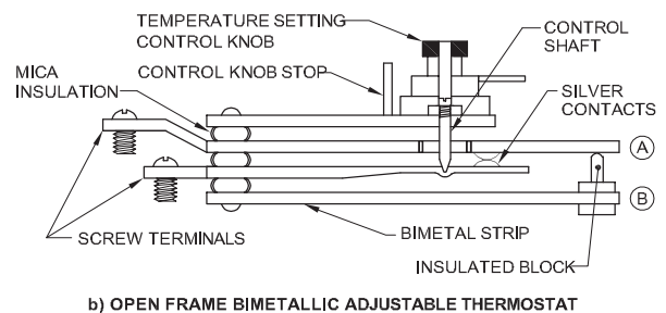
b) OPEN FRAME BIMETALLIC ADJUSTABLE THERMOSTAT
