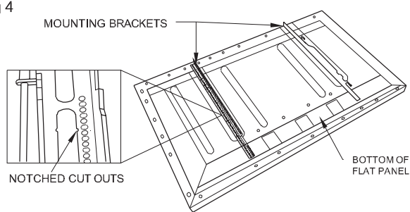
MOUNTING BRACKET INSTALLATION
