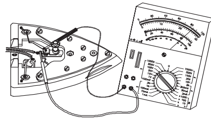
(A) TESTING THE THERMOSTAT FOR CONTINUITY
