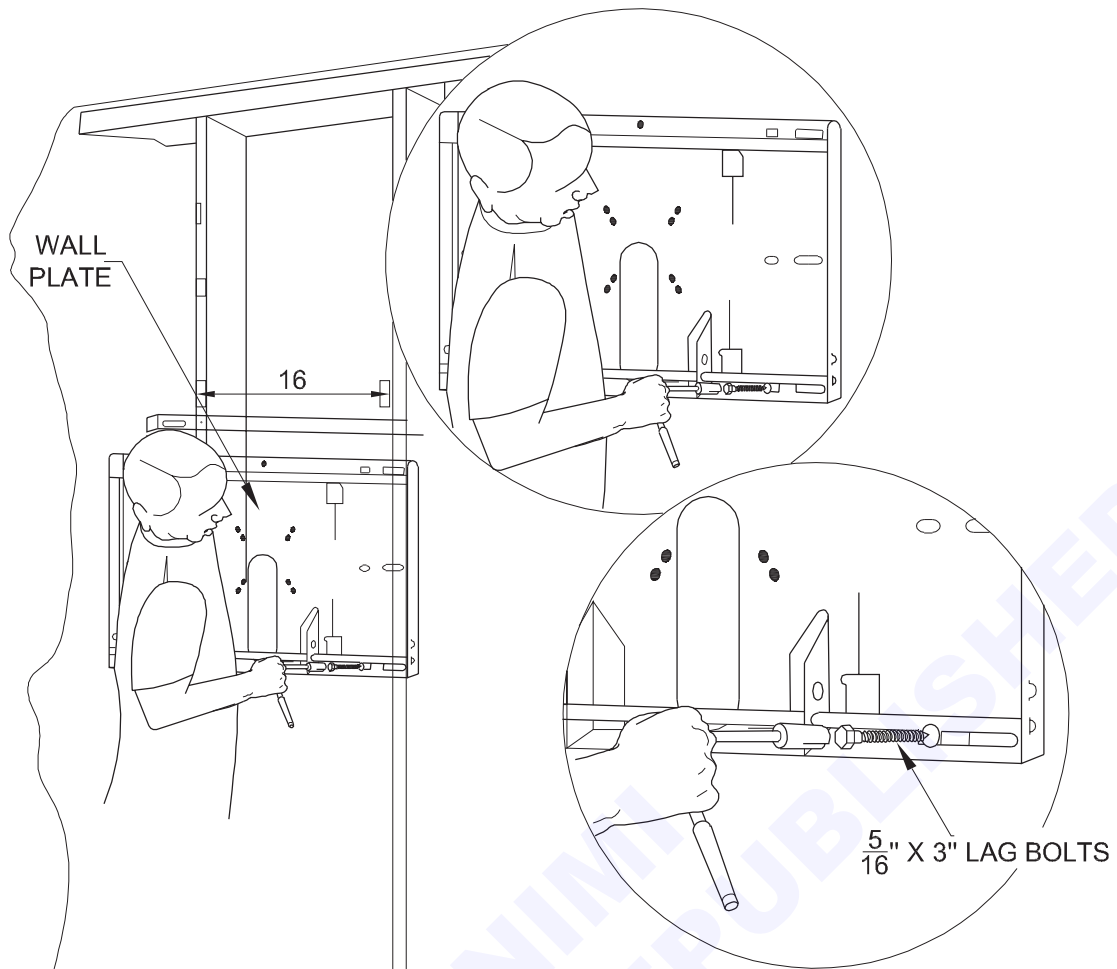
WOOD INSTALLATION
