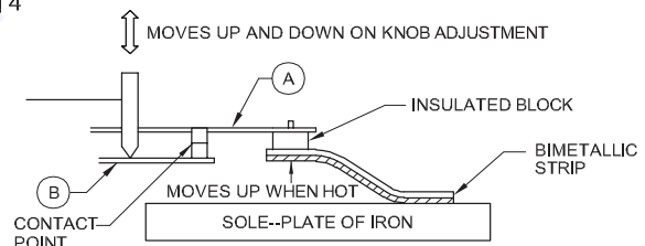
a) A SIMPLIFIED SKETCH OF ADJUSTABLE THERMOSTAT
