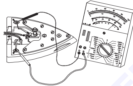
(B) TESTING THE HEATING ELEMENT FOR CONTINUITY
