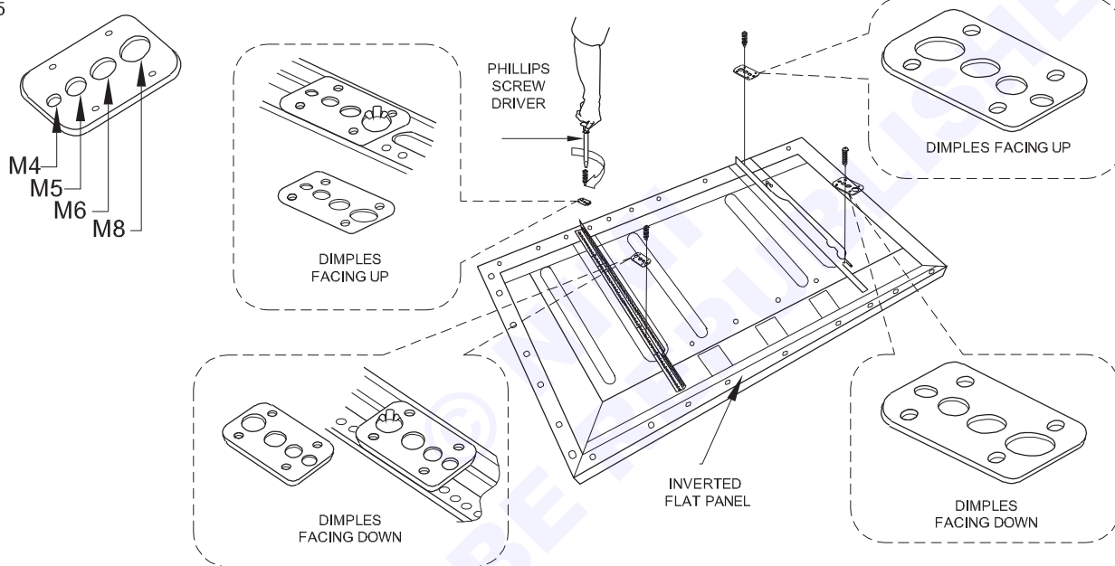
MOUNTING BRACKET INSTALLATION
