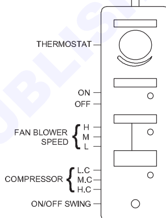
CORD REMOTE
