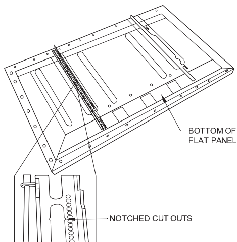
MOUNTING BRACKET INSTALLATION
