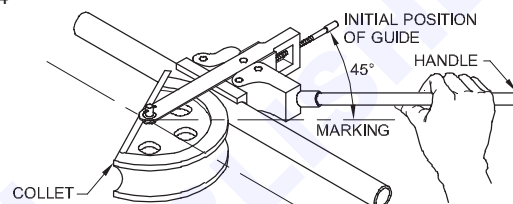
OPERATING A PIPE BENDING MACHINE
