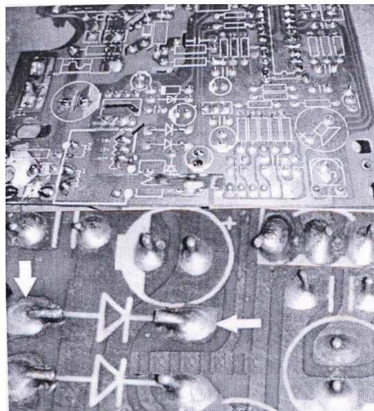
DRY SOLDERS
