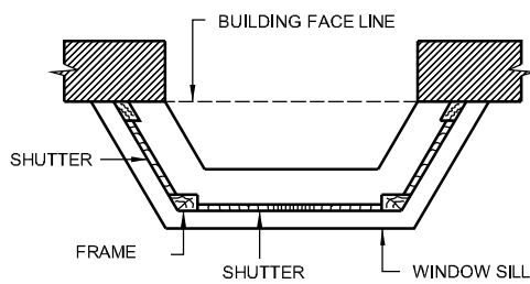
SPLOYED BAY WINDOW
