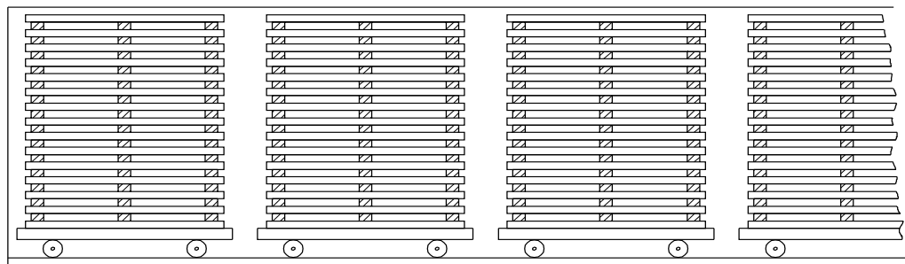
PROGRESSIVE KILN IS SIMILAR TO AN ASSEMBLY LINE. A CARLOAD OF LUMBER ENTERS THE KILN AND GOES THROUGH EACH OF SEVERAL DRYING COMPARTMENTS, STAGES OF DRYING
