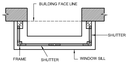
SQUARE BAY WINDOW
