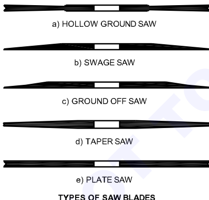
TYPES OF SAW BLADES
