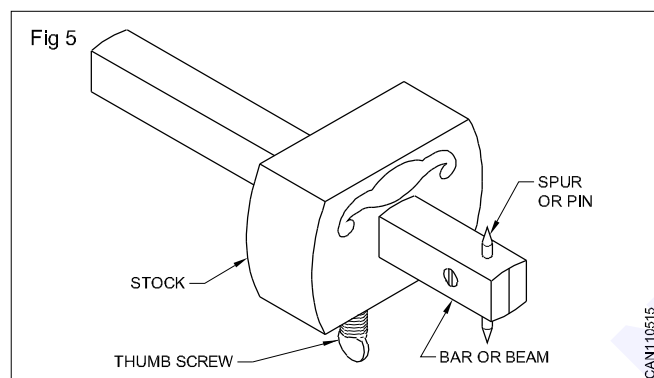
Marking gauge (Fig 5)
