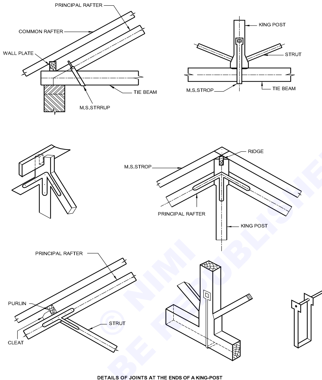
DETAILS OF JOINTS AT THE ENDS OF A KING-POST
