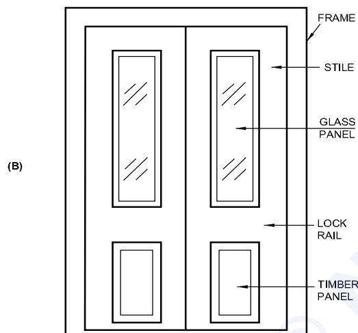
PARTLY PANELLED AND PARTLY DOOR
