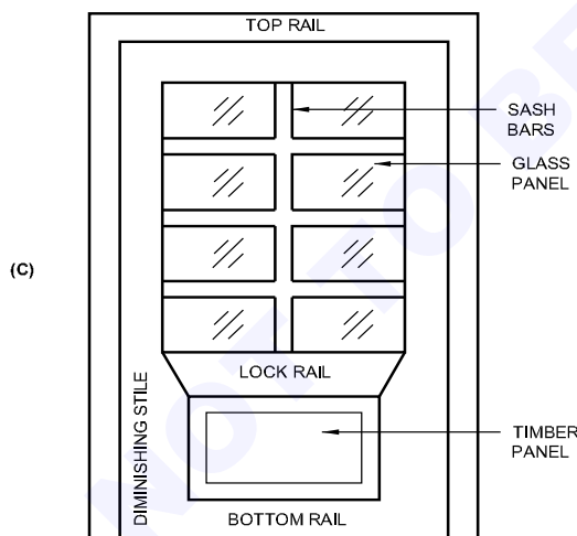
DOOR WITH DIMINISHING STYLES GLAZE DOOR
