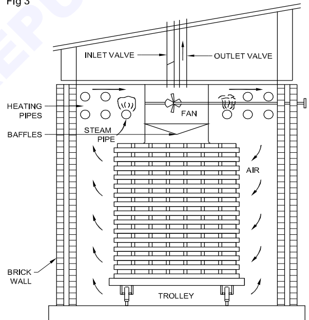
CROSS SECTION OF DRY KILN
