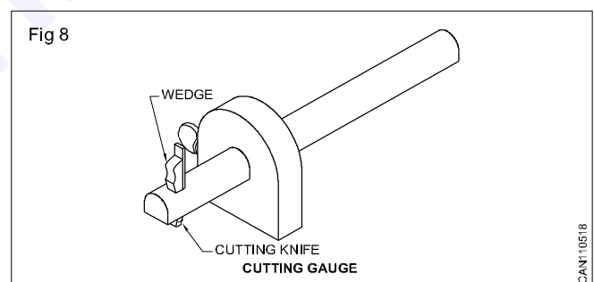
Cutting gauge (Fig 8)
