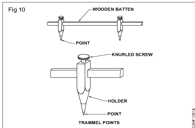
Trammel points (Fig 10)
