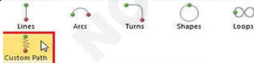
Fig 80 Motion Paths
