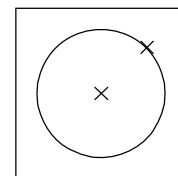
CIRCLE COMMAND
