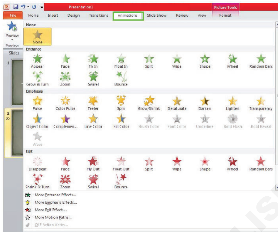
Animation effects
