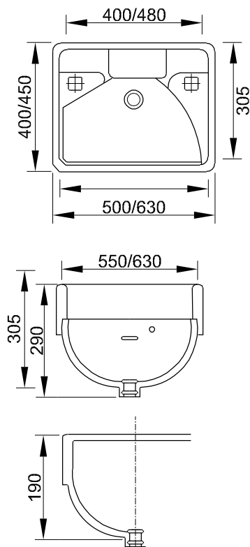
PLAN,SECTION AND SIDE SECTION OF FLAT BACK WASH BASIN
