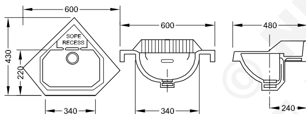
PLAN,SECTION AND SIDE SECTION OF ANGLE WASH-BASIN
