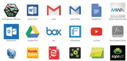
Application software
