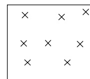
POINT COMMAND
