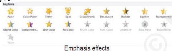
Emphasis effects
