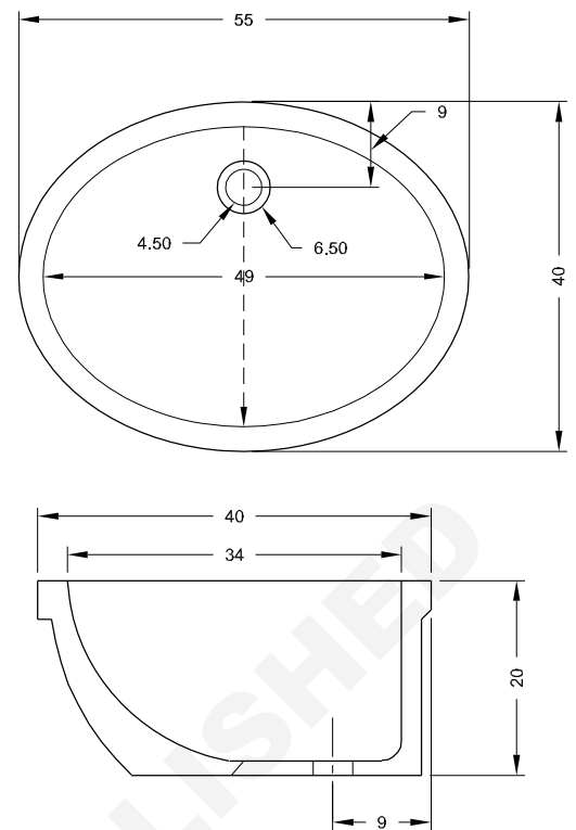
PLAN AND SECTION OF OVAL WASH-BASIN
