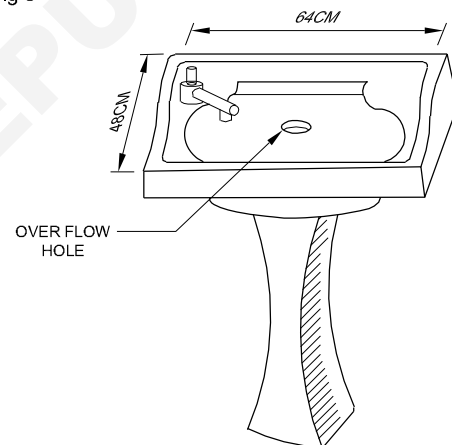
PEDESTAL WASH BASIN
